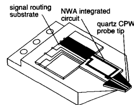
Fig. 2. Active probe hybrid assembly.
