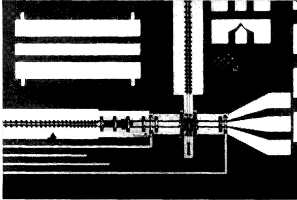
Fig. 4. Photograph of a fabricated network analyzer IC.
